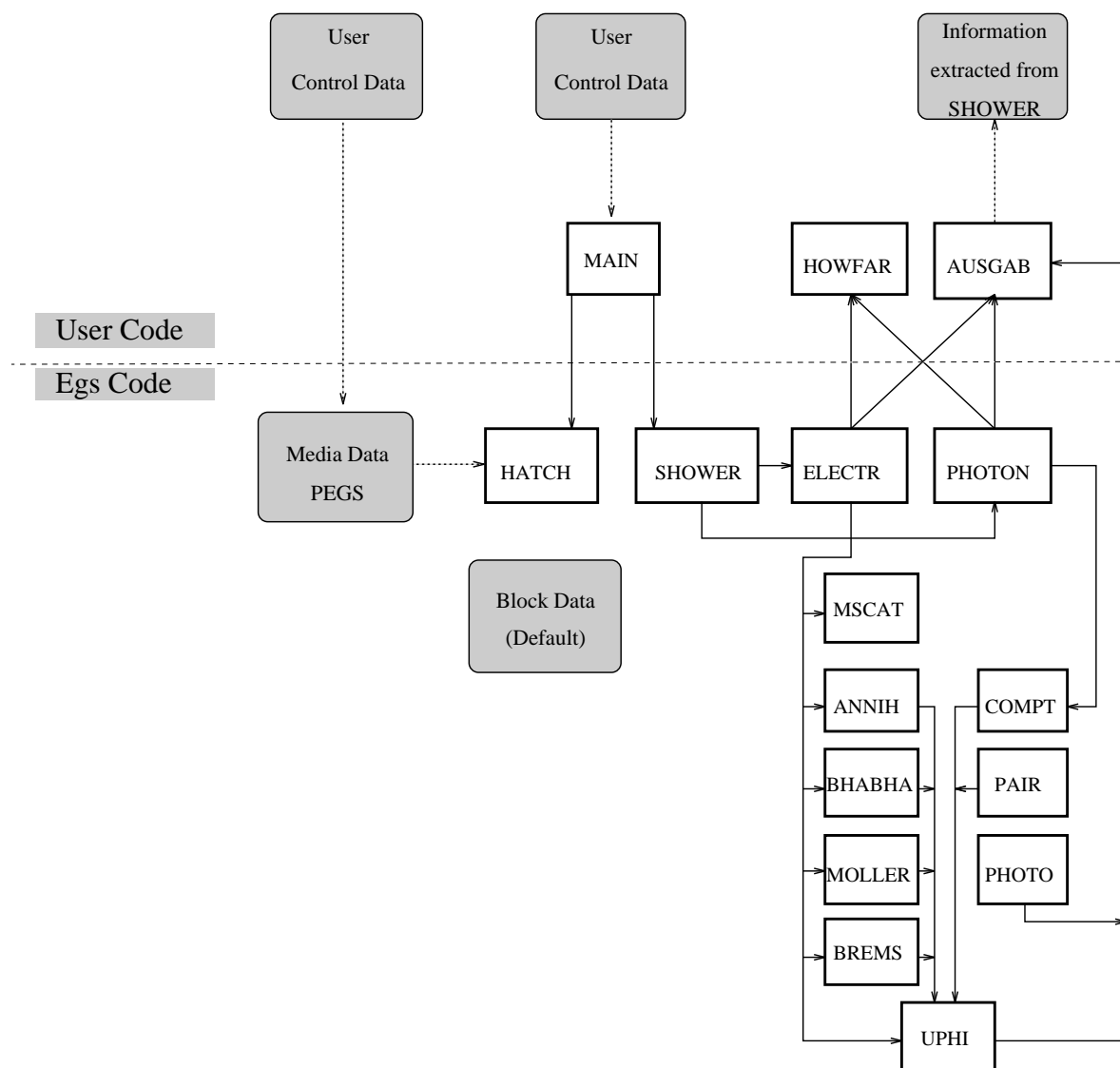
Figure 1: Division between user-interface and EGS4.
